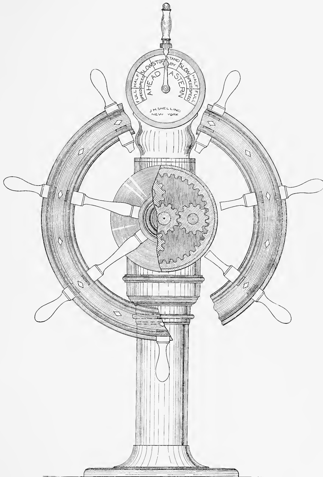
SNELLING'S COMBINED HAND STEERER AND ENGINE-ROOM TELEGRAPH.
